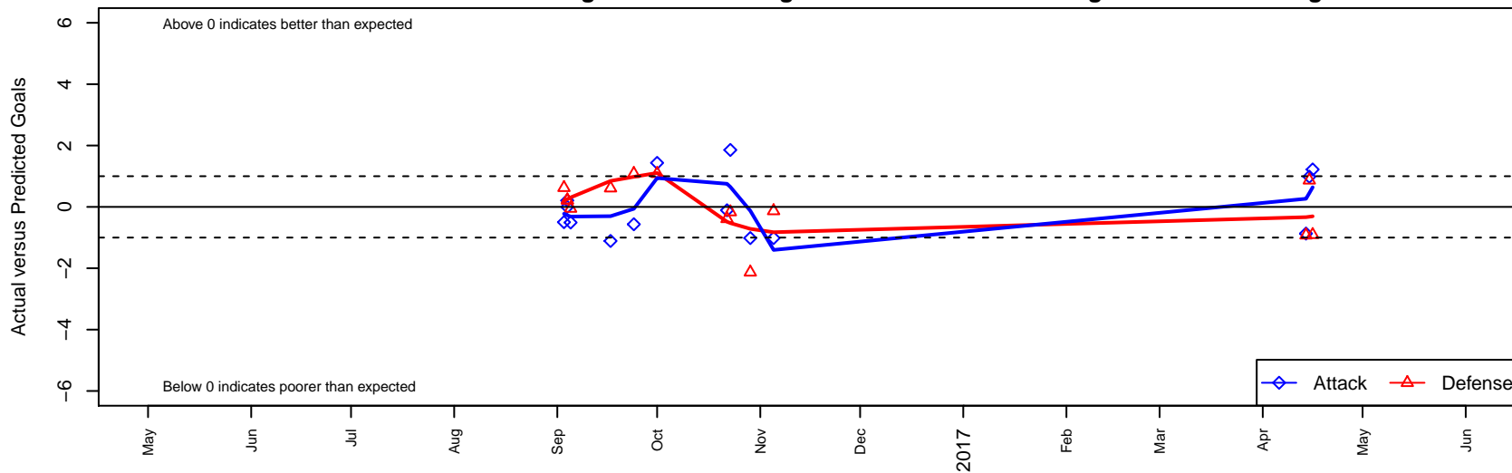
Surrey United B01 Dots are actual minus expected GF (blue circles) and GA (red triangles). Blue line is smoothed change in attack strength. Red is smoothed change in defense strength.
